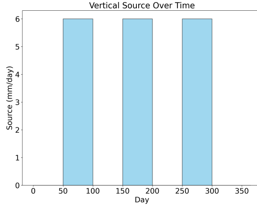
Figure 6: Time-varying vertical recharge applied over 365 days.
